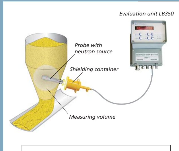
Moisture measurement with bunker probe
